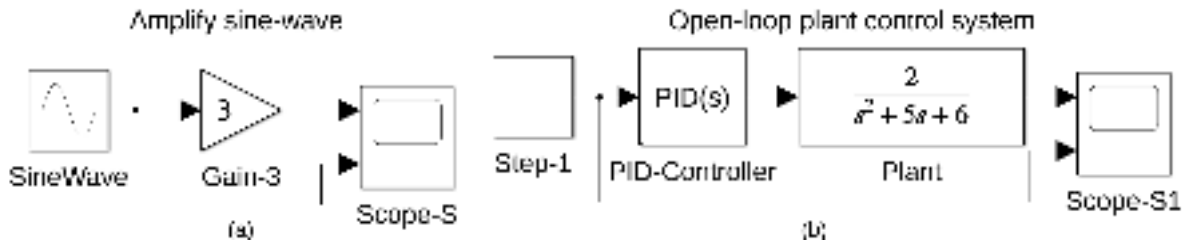
Figure 2.9. Two tiny example Simulink models.
