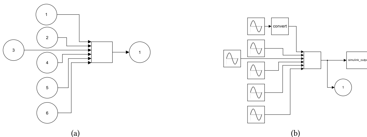
Figure 4.18. Our black box wrapping setup: all model inports in Figure 4.18a are replaced by signal generators in Figure 4.18b. The first port of this example model is of type boolean and a boolean converter is thus added. Similarly, all output signals are tapped into with a To Workspace Block to record the model output.
